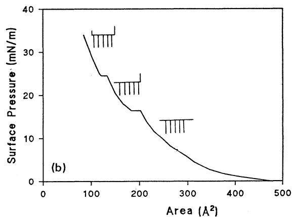
FIG. 2. Surface-pressure-molecular-area isotherms of (a) crown ether liquid crystal and (b) polymer liquid-crystal monolayers on the air-water interface at 25°C. The molecular conformations in the corresponding phases are also schematically illustrated.
